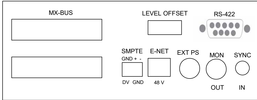
FIGURE 2-6. Control Backplane
