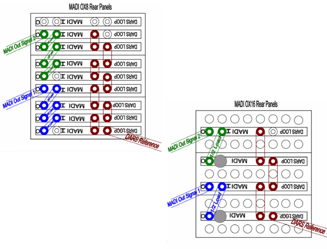
FIGURE E-6. MADI Output rear panel cabling
