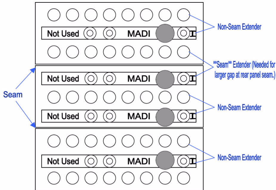
FIGURE E-2. Seam and Non-Seam slot installation - Input
